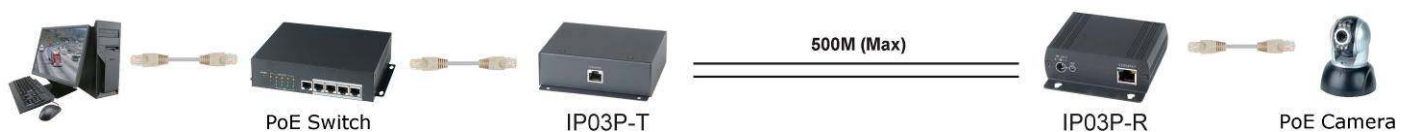
IP03PT with POE switch power input to IP03R and POE camera
