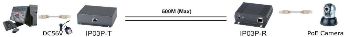
IP03PT with DC 48/56V Power adapter power input to IP03R and POE camera
